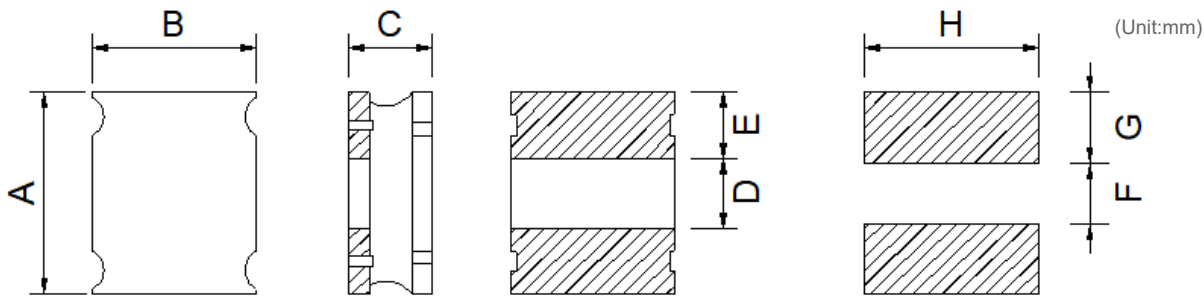
Recommended Land Pattern 推荐焊盘
