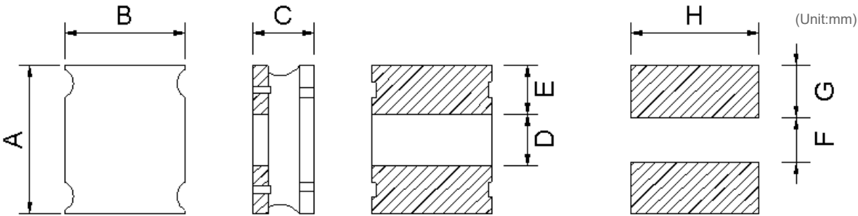
Recommended Land Pattern 推荐焊盘
