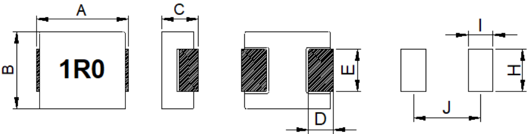
Recommended Land Pattern 推荐焊盘
